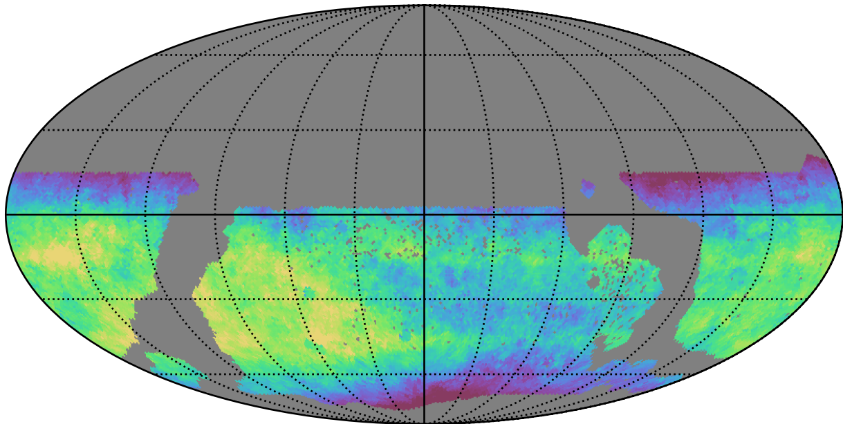
too_100_1v3.4_10yrs WFD i band: Median fiveSigmaDepth
