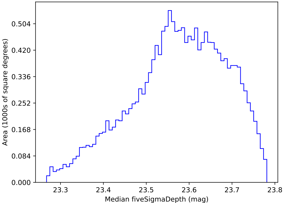
too_100_1v3.4_10yrs WFD i band: Median fiveSigmaDepth
