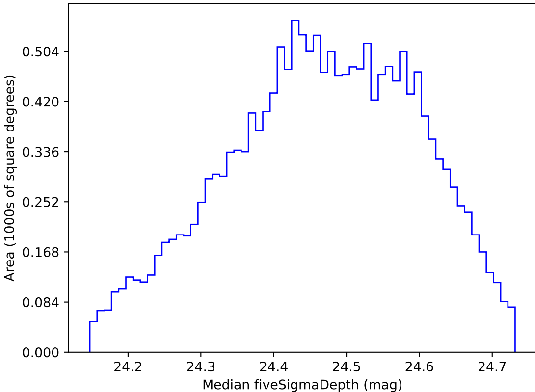
too_100_1v3.4_10yrs WFD g band: Median fiveSigmaDepth
