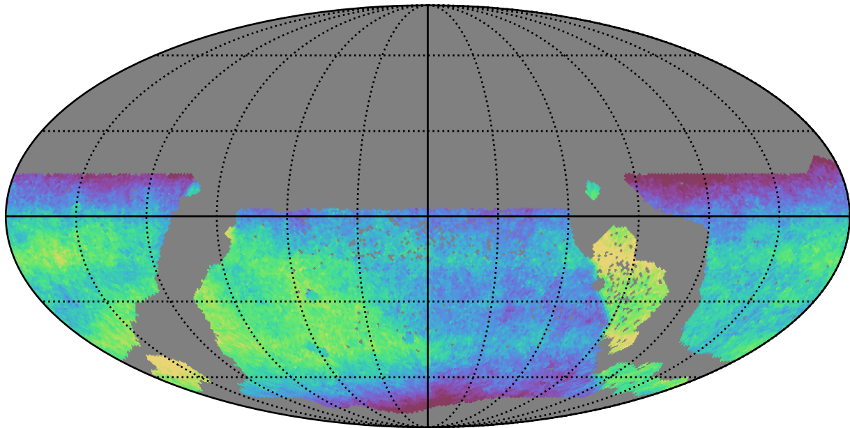
too_100_1v3.4_10yrs WFD all bands: Median fiveSigmaDepth
