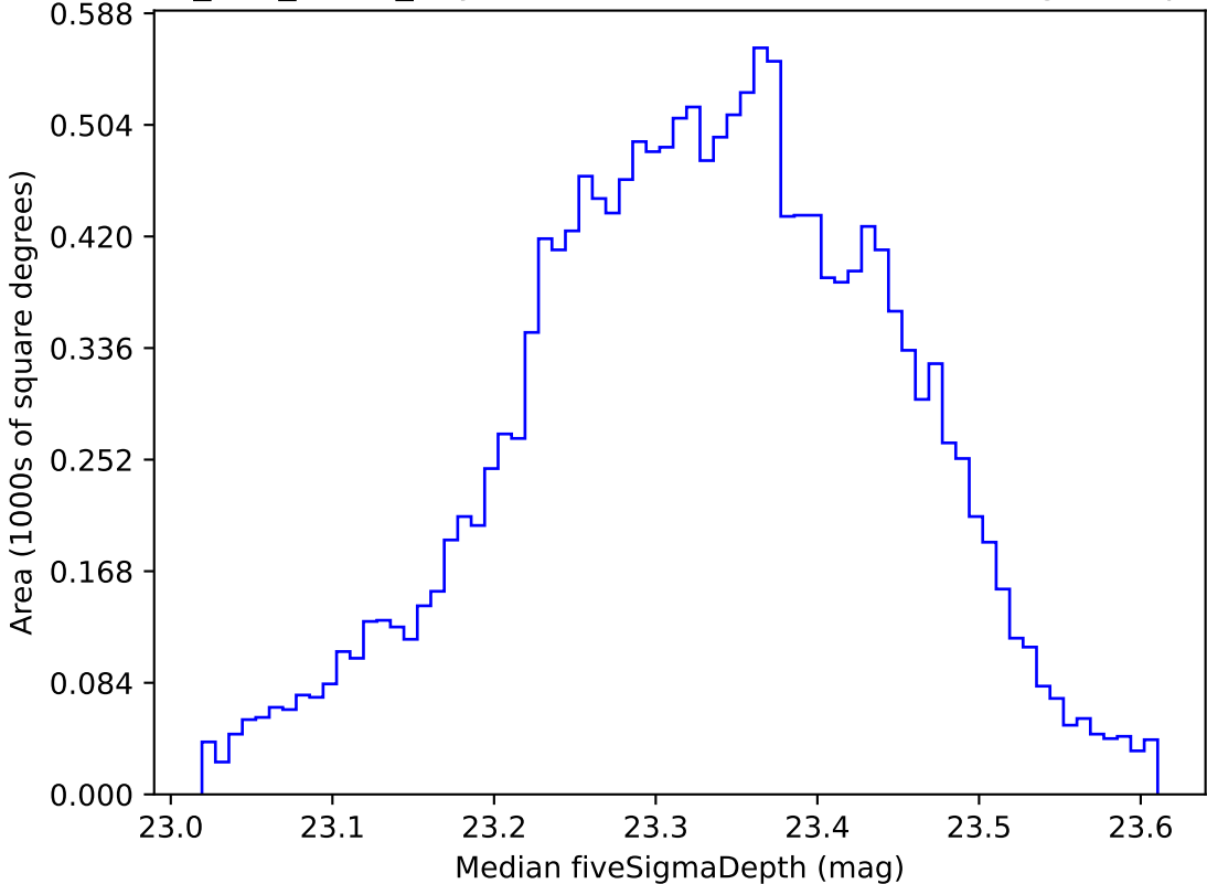
too_100_1v3.4_10yrs WFD all bands: Median fiveSigmaDepth
