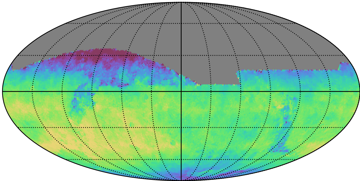
too_100_1v3.4_10yrs All sky z band: Median fiveSigmaDepth
