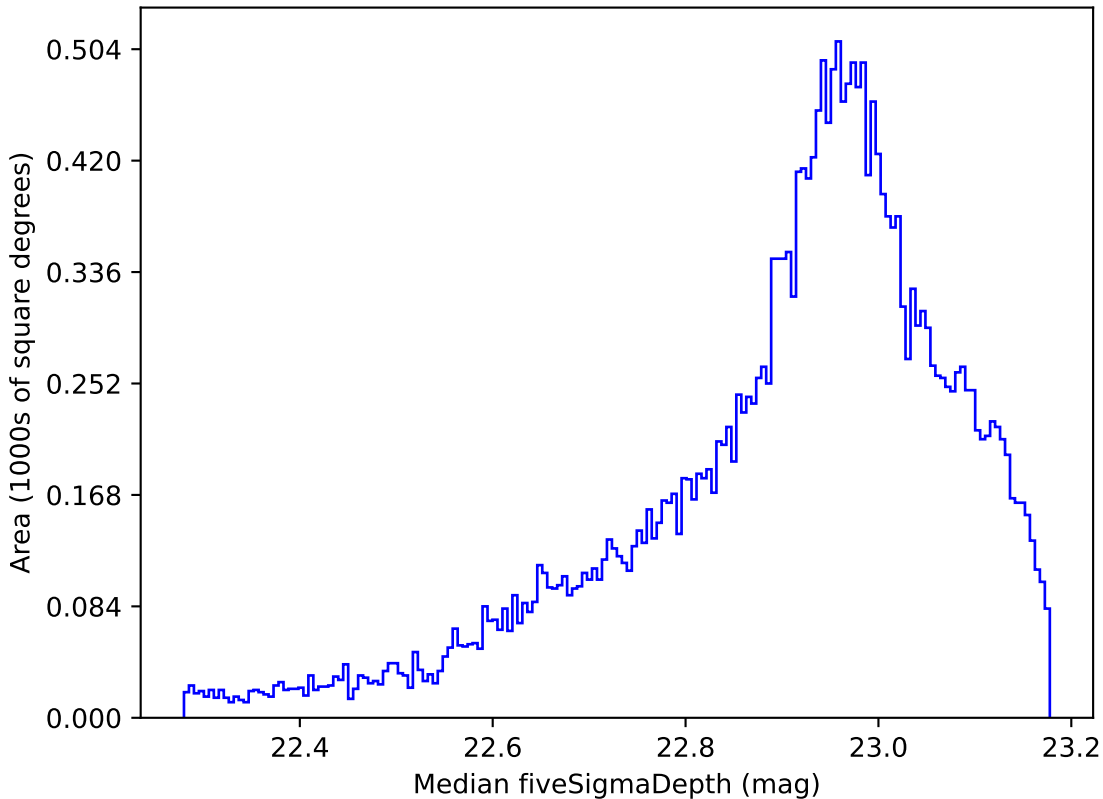
too_100_1v3.4_10yrs All sky z band: Median fiveSigmaDepth
