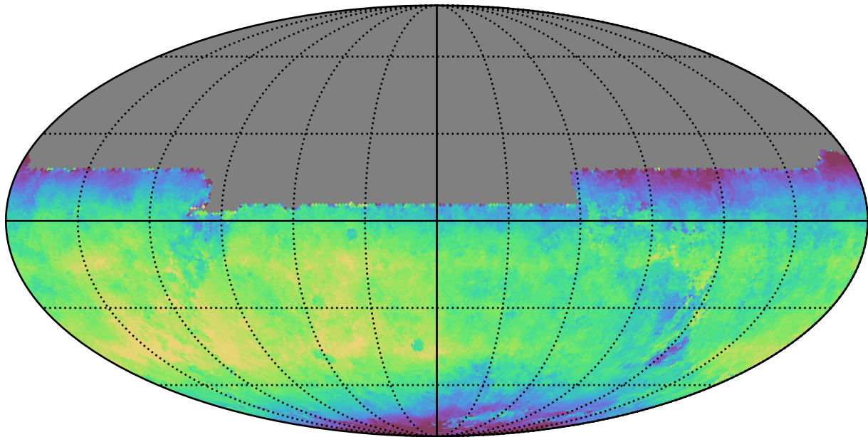
too_100_1v3.4_10yrs All sky y band: Median fiveSigmaDepth
