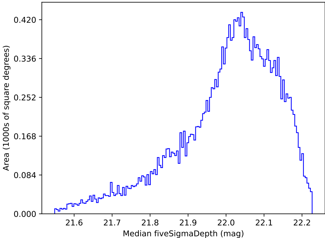
too_100_1v3.4_10yrs All sky y band: Median fiveSigmaDepth
