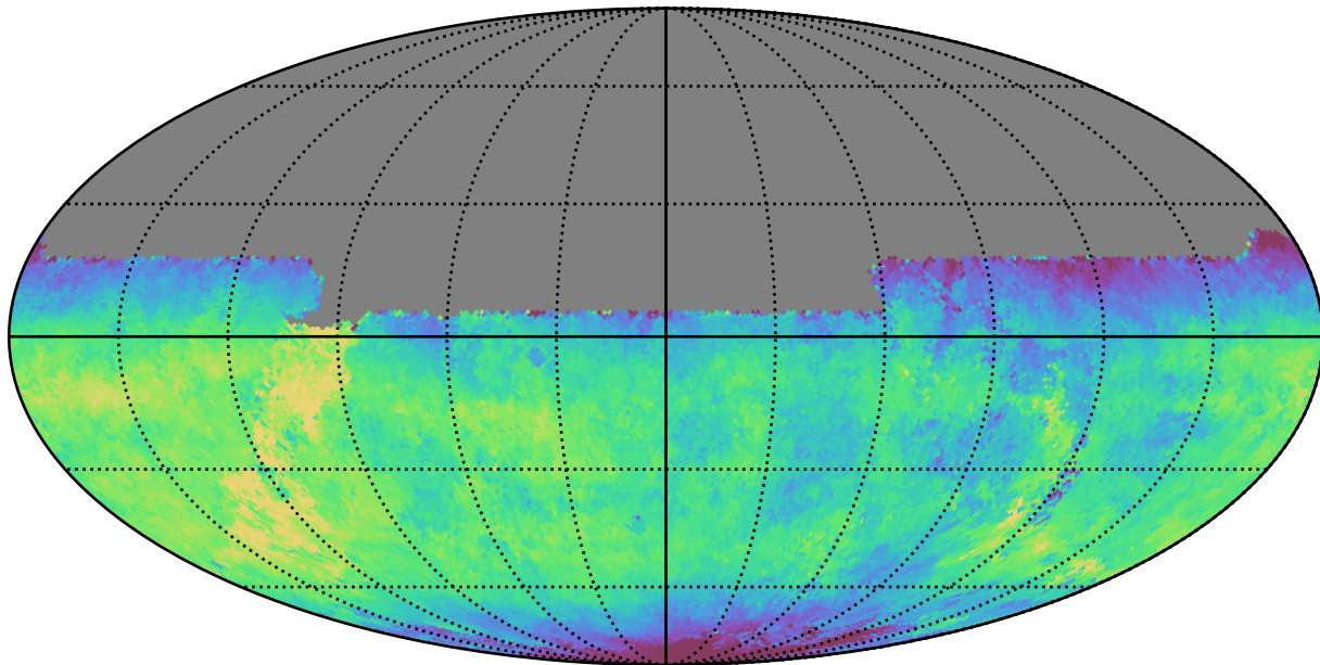
too_100_1v3.4_10yrs All sky u band: Median fiveSigmaDepth
