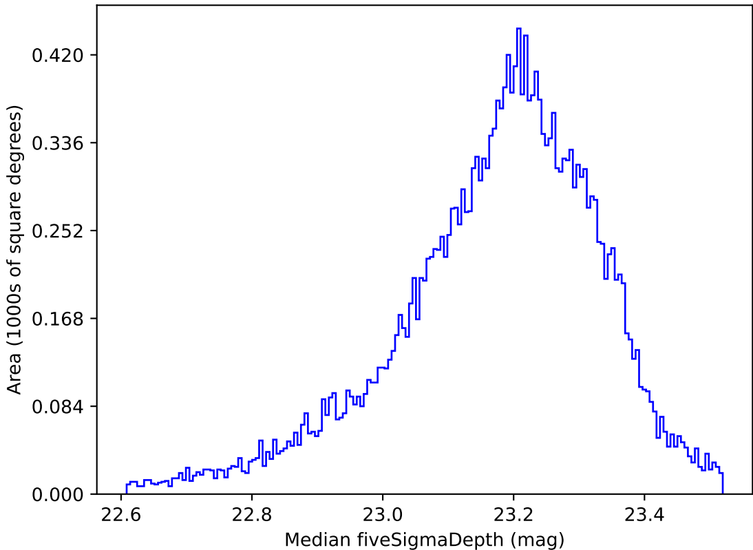
too_100_1v3.4_10yrs All sky u band: Median fiveSigmaDepth
