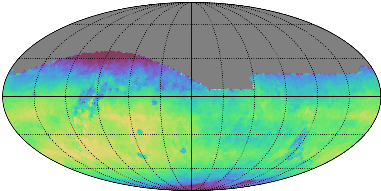
too_100_1v3.4_10yrs All sky r band: Median fiveSigmaDepth
