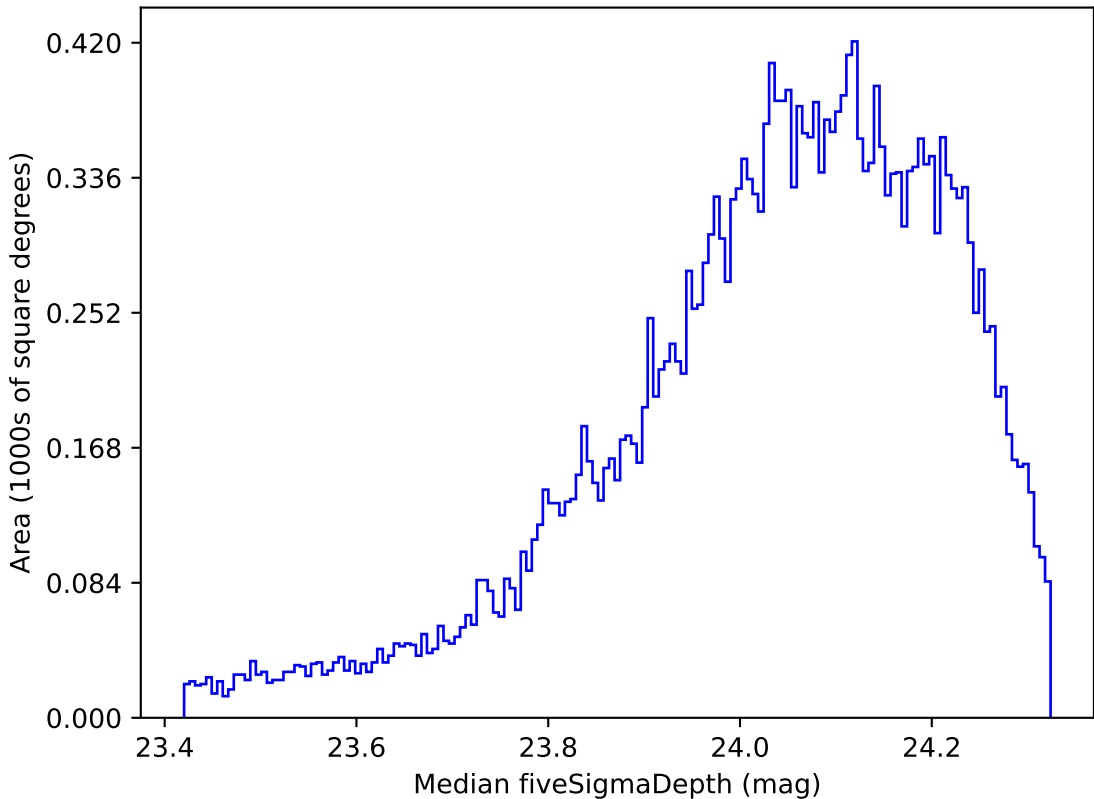
too_100_1v3.4_10yrs All sky r band: Median fiveSigmaDepth
