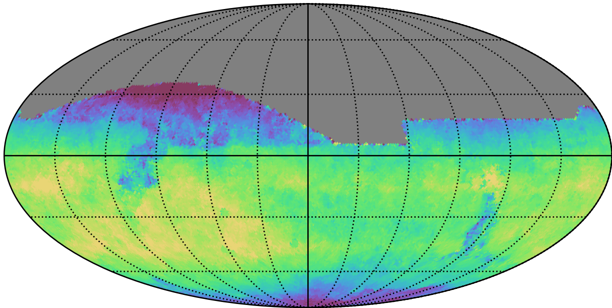
too_100_1v3.4_10yrs All sky i band: Median fiveSigmaDepth
