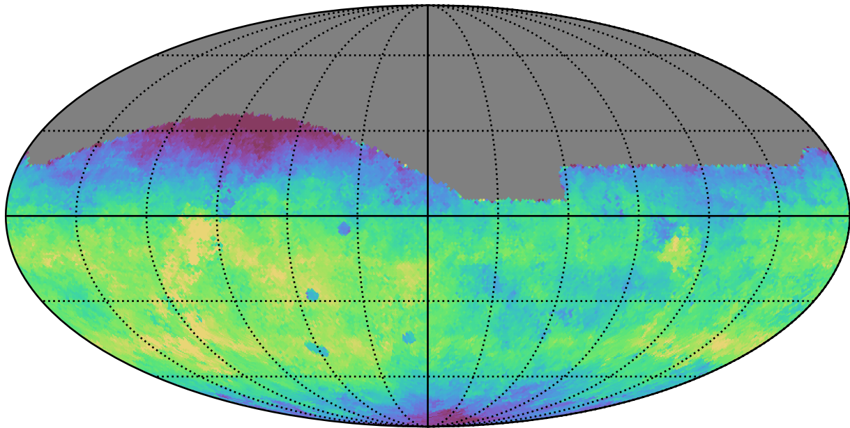
too_100_1v3.4_10yrs All sky g band: Median fiveSigmaDepth
