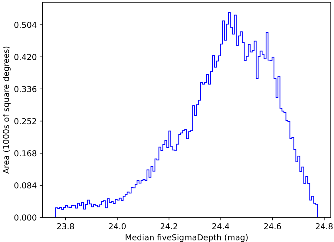
too_100_1v3.4_10yrs All sky g band: Median fiveSigmaDepth
