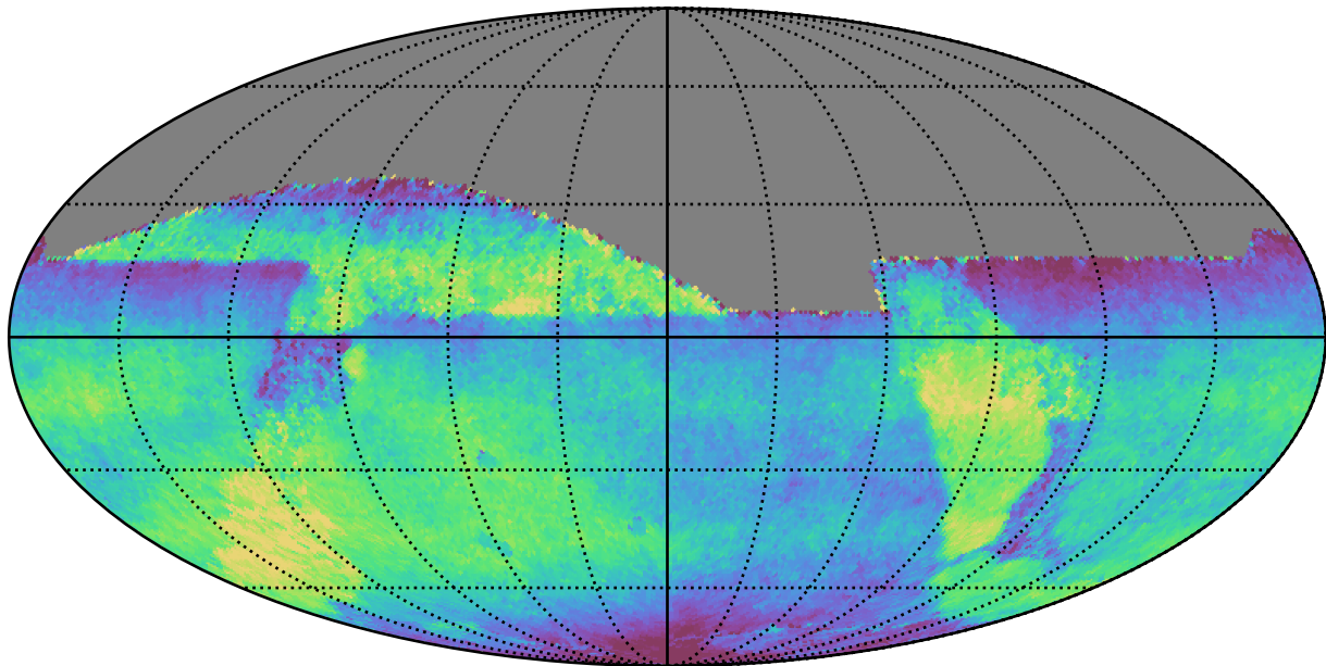
too_100_1v3.4_10yrs All sky all bands: Median fiveSigmaDepth
