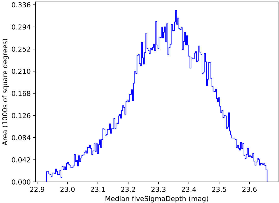
too_100_1v3.4_10yrs All sky all bands: Median fiveSigmaDepth
