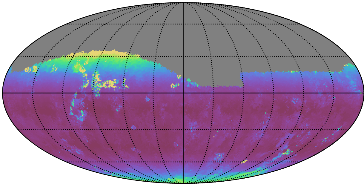
too_100_1v3.4_10yrs Yr 1 z band: Median airmass
