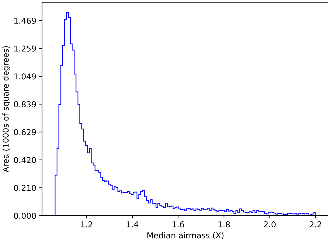
too_100_1v3.4_10yrs Yr 1 z band: Median airmass
