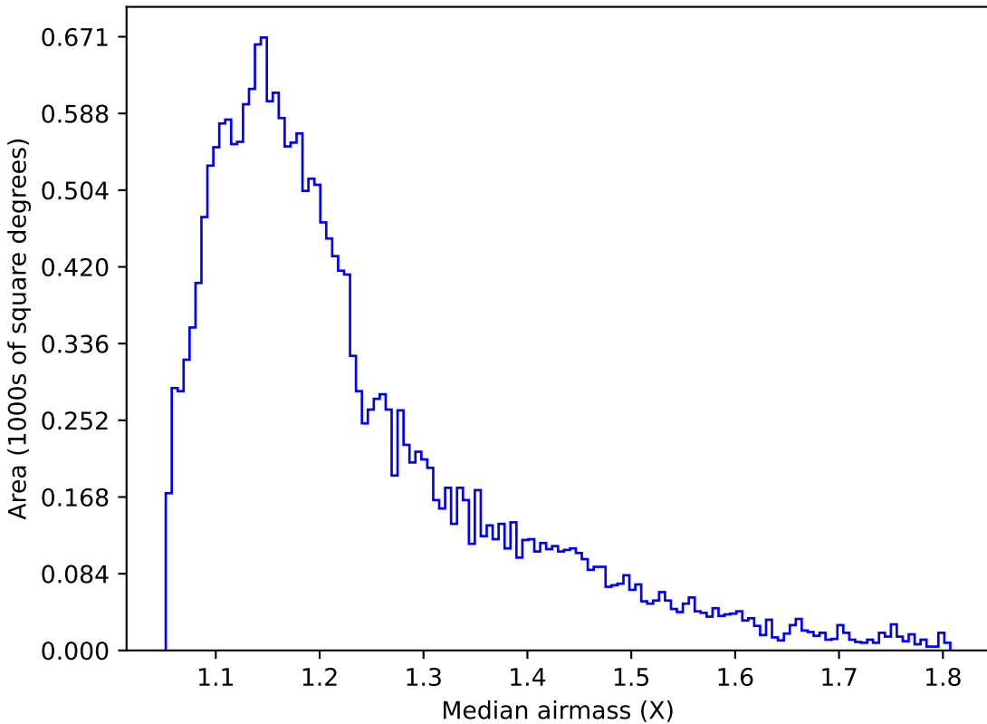
too_100_1v3.4_10yrs Yr 1 u band: Median airmass
