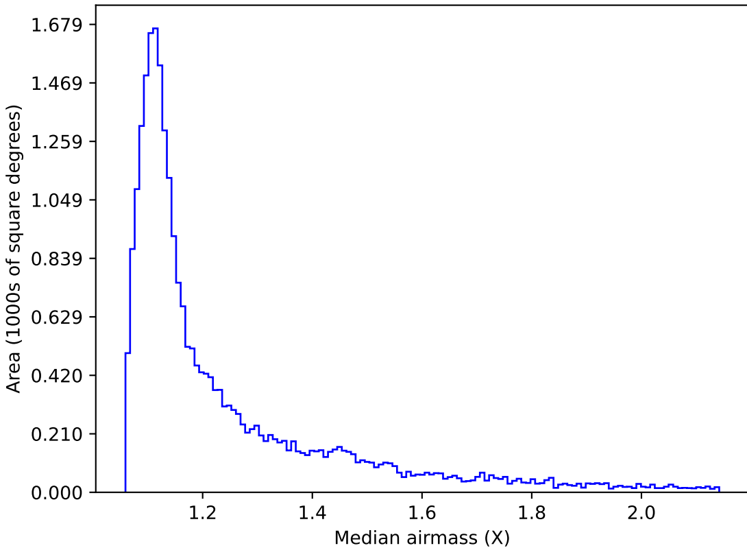
too_100_1v3.4_10yrs Yr 1 r band: Median airmass
