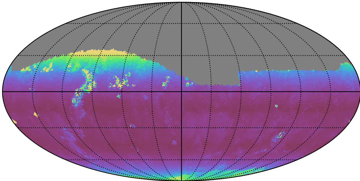
too_100_1v3.4_10yrs Yr 1 i band: Median airmass
