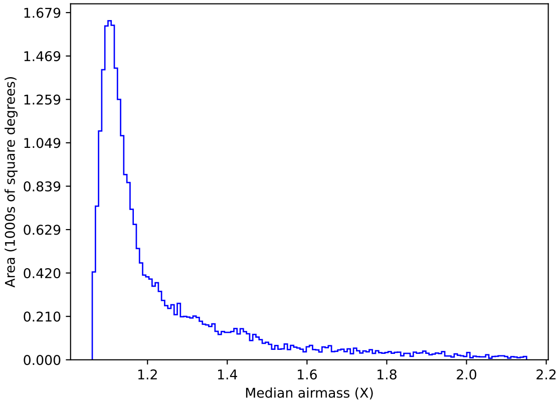
too_100_1v3.4_10yrs Yr 1 i band: Median airmass
