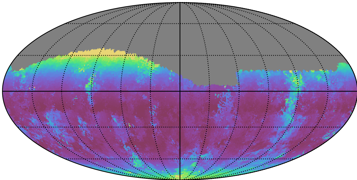
too_100_1v3.4_10yrs Yr 1 g band: Median airmass
