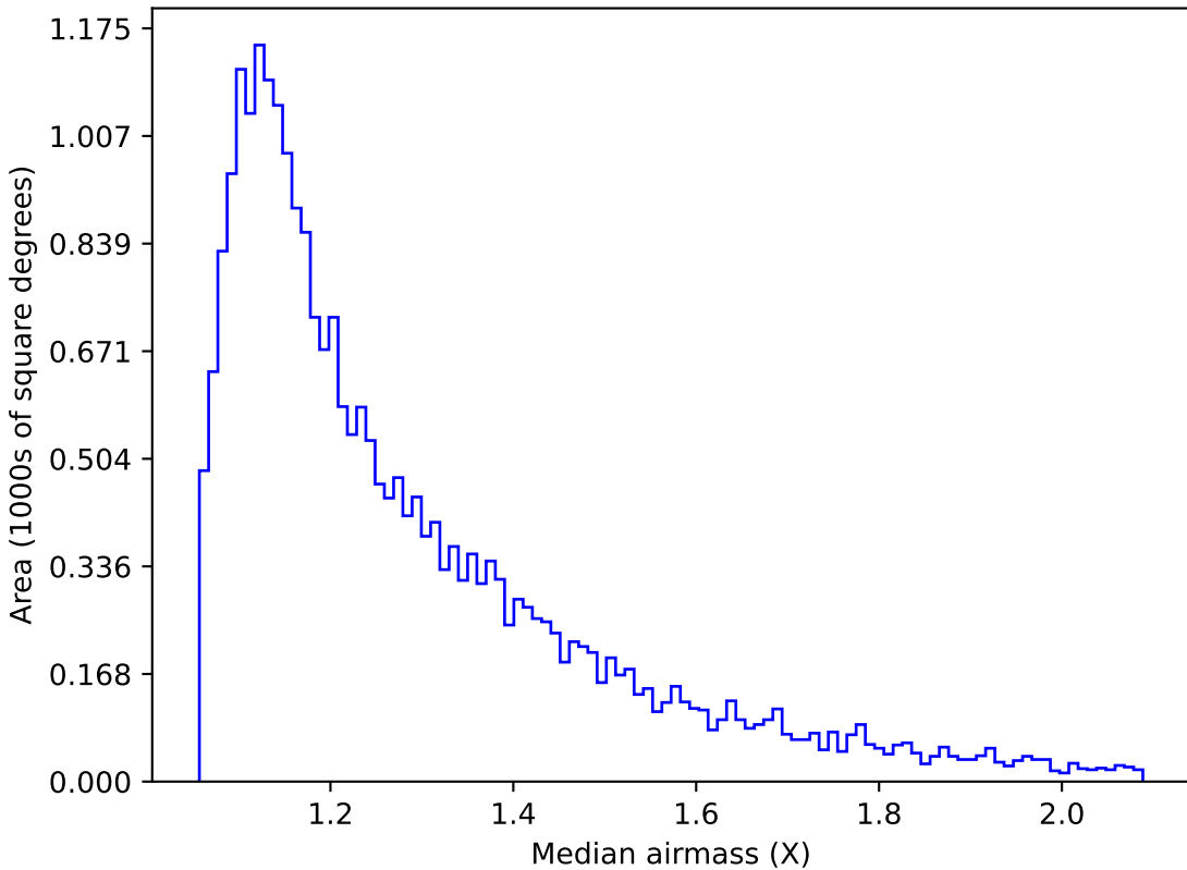
too_100_1v3.4_10yrs Yr 1 g band: Median airmass
