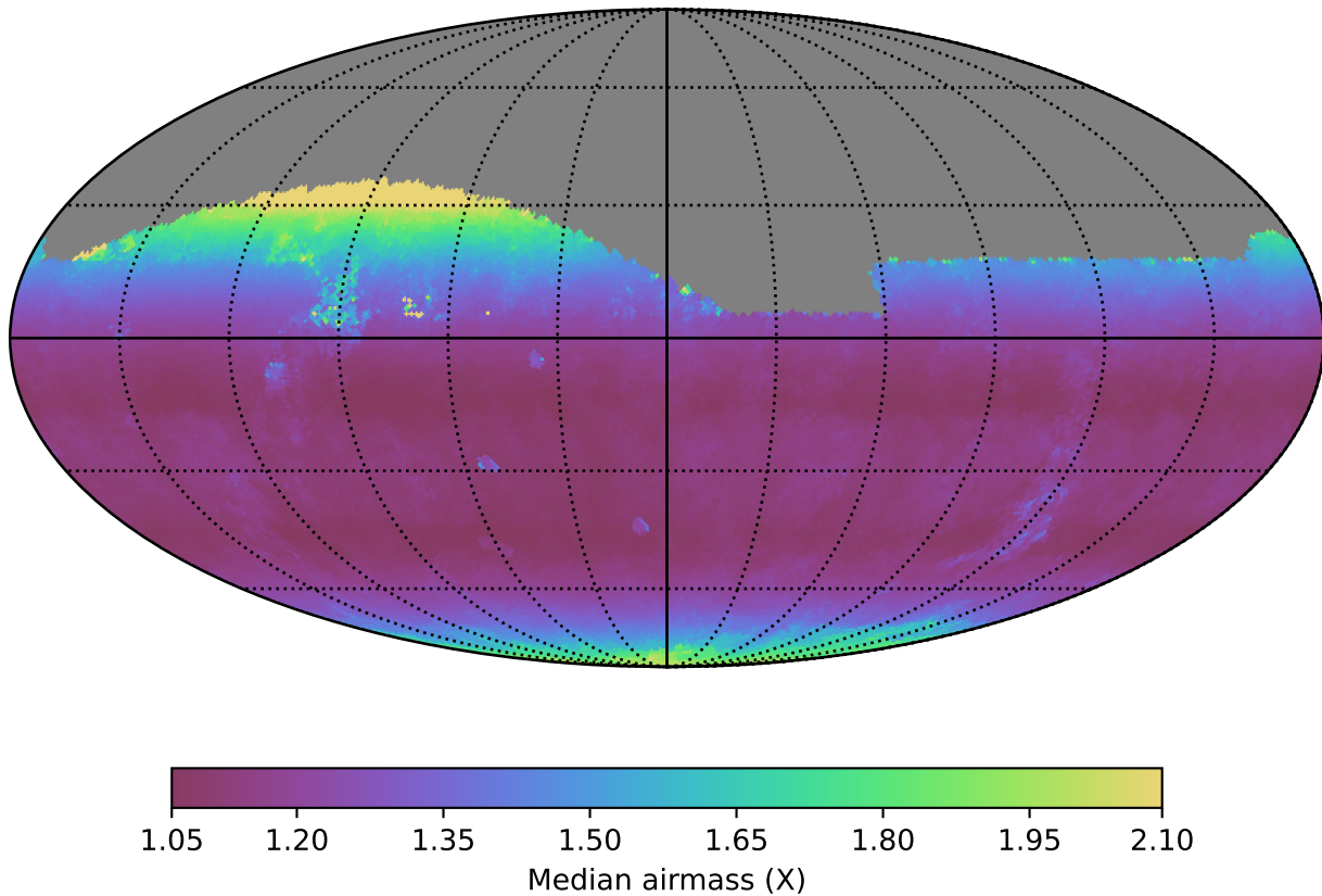
too_100_1v3.4_10yrs Yr 1 all bands: Median airmass
