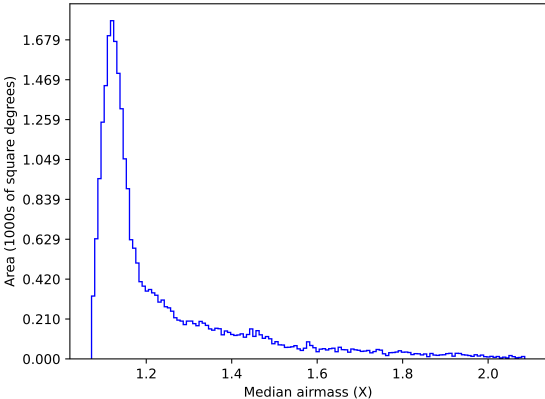
too_100_1v3.4_10yrs Yr 1 all bands: Median airmass
