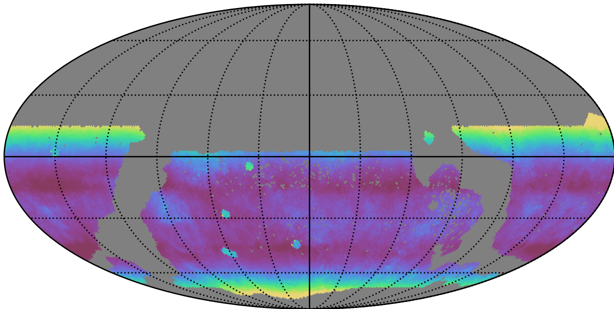
too_100_1v3.4_10yrs WFD z band: Median airmass
