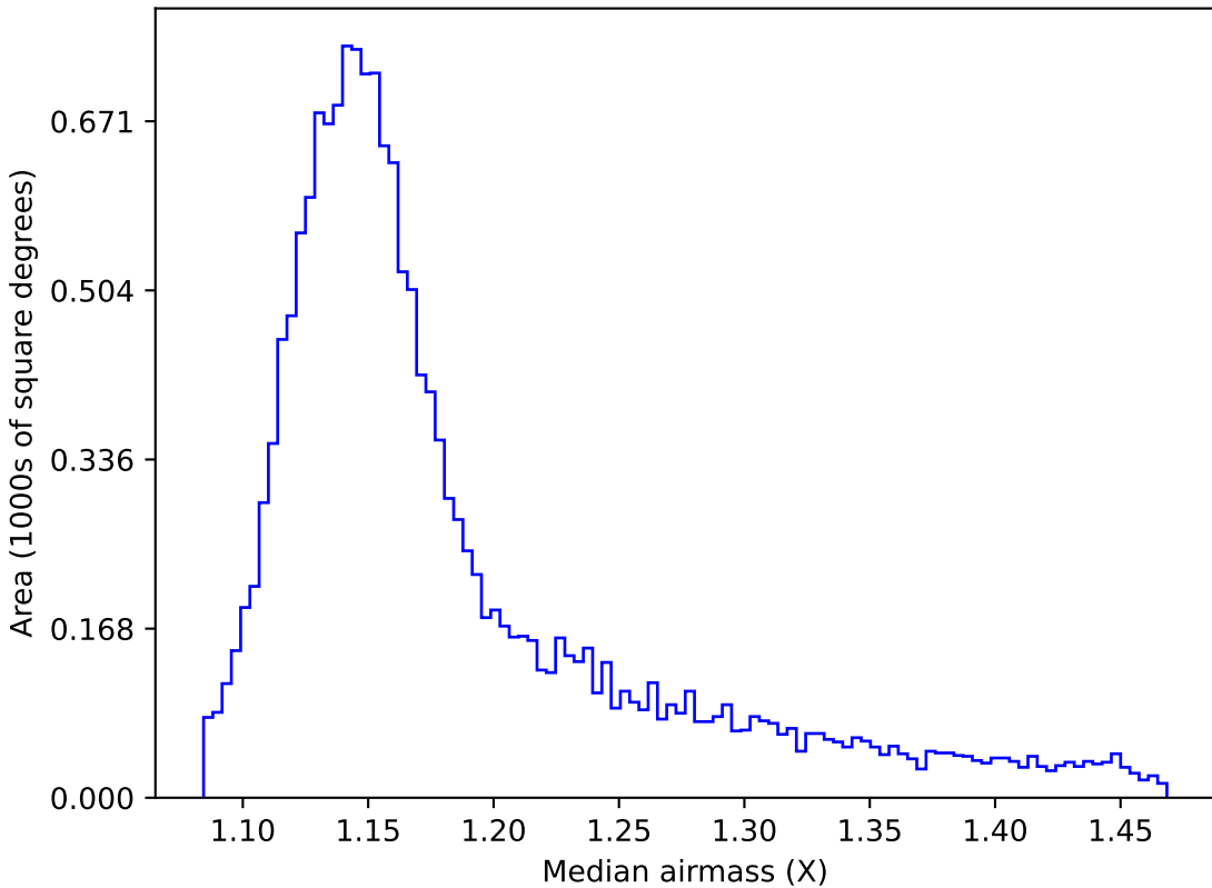
too_100_1v3.4_10yrs WFD z band: Median airmass
