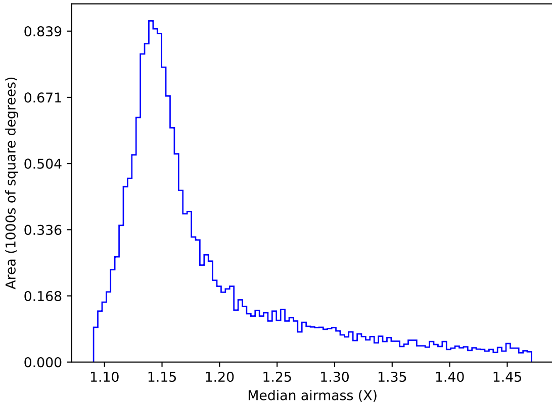
too_100_1v3.4_10yrs WFD y band: Median airmass
