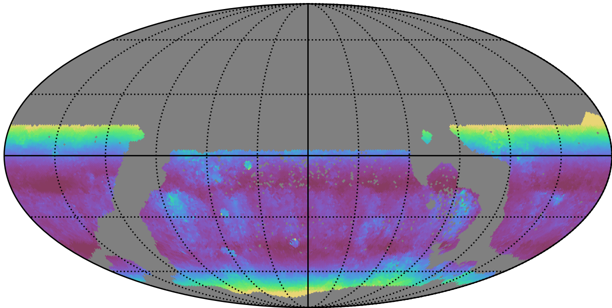
too_100_1v3.4_10yrs WFD u band: Median airmass
