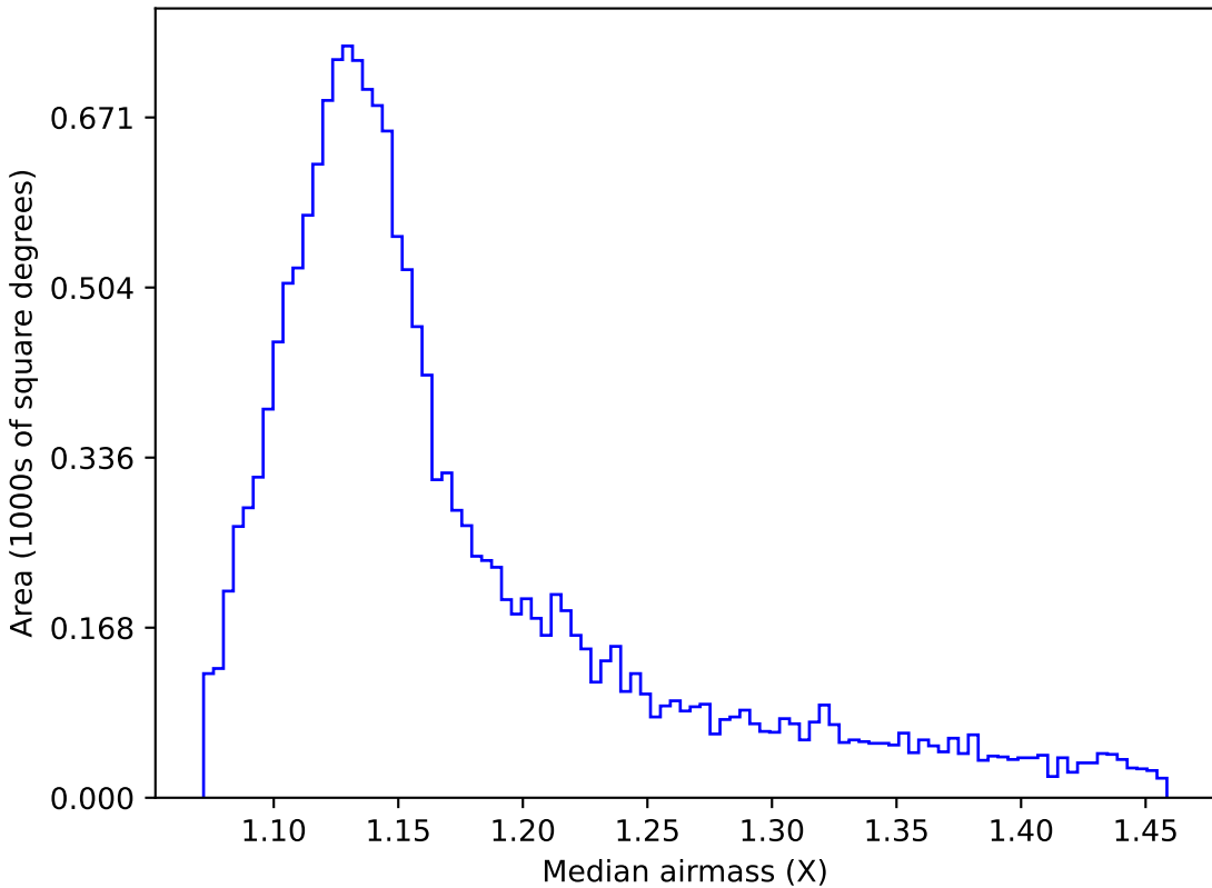
too_100_1v3.4_10yrs WFD u band: Median airmass
