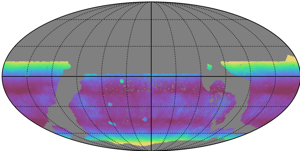
too_100_1v3.4_10yrs WFD r band: Median airmass
