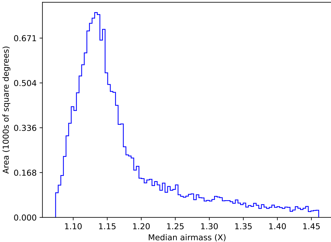
too_100_1v3.4_10yrs WFD r band: Median airmass
