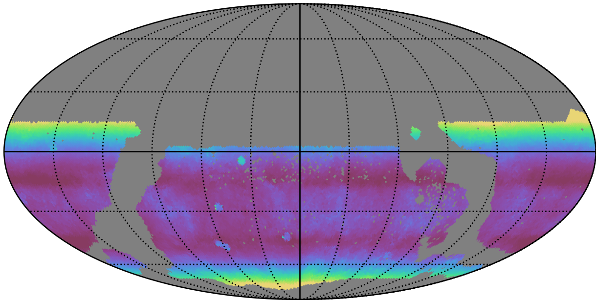
too_100_1v3.4_10yrs WFD i band: Median airmass
