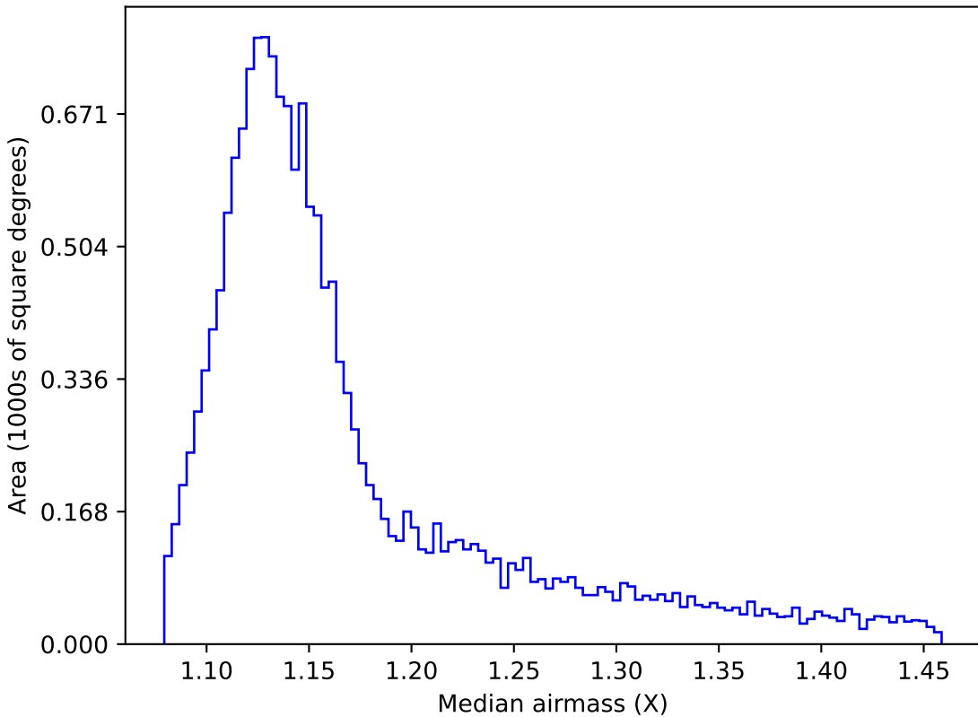
too_100_1v3.4_10yrs WFD i band: Median airmass
