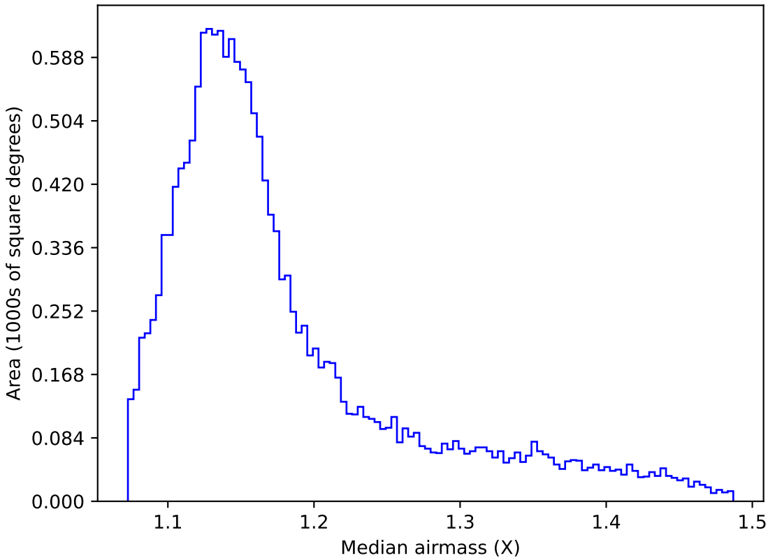
too_100_1v3.4_10yrs WFD g band: Median airmass
