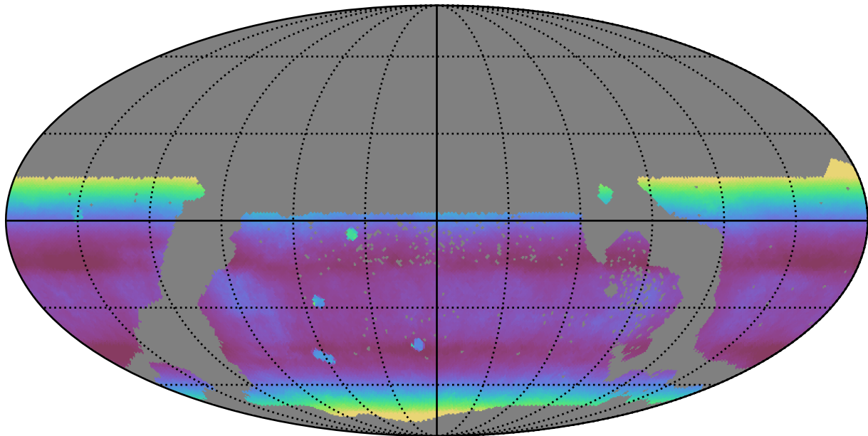
too_100_1v3.4_10yrs WFD all bands: Median airmass
