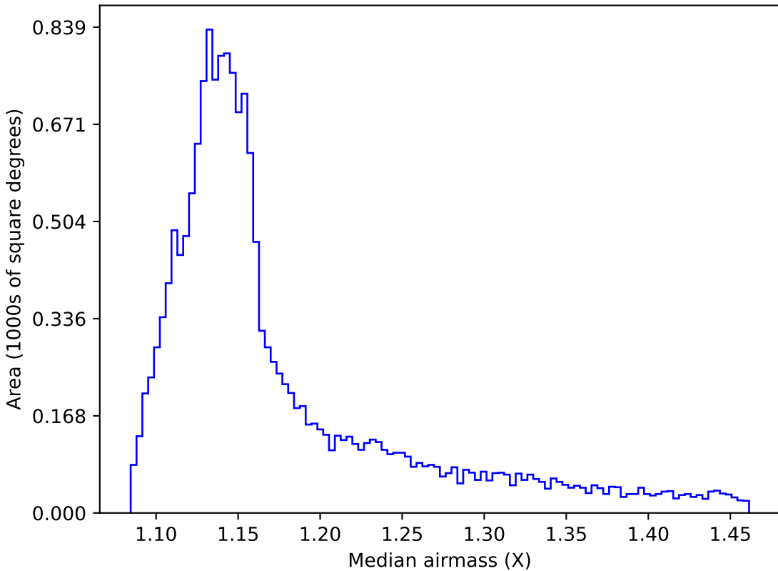
too_100_1v3.4_10yrs WFD all bands: Median airmass
