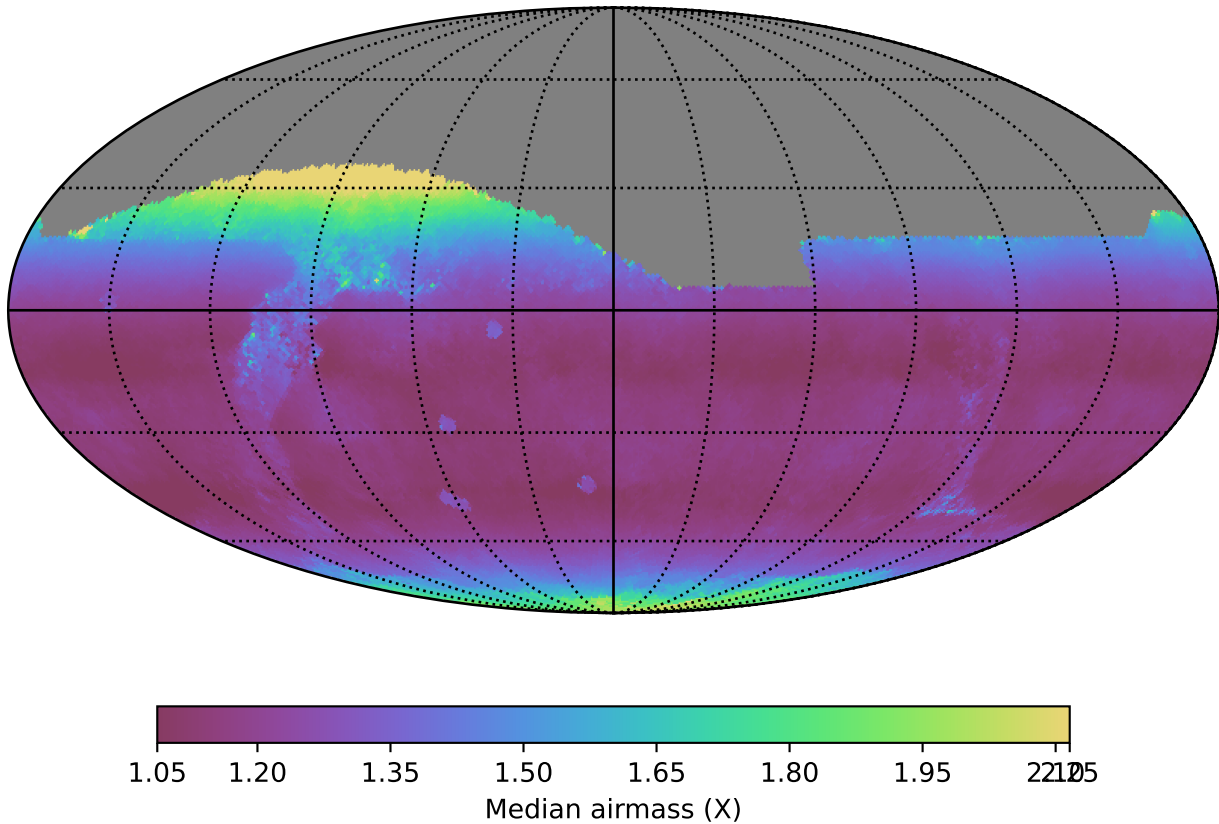
too_100_1v3.4_10yrs All sky z band: Median airmass
