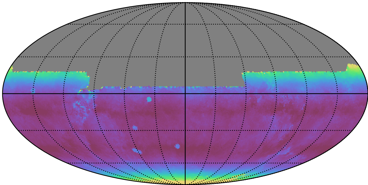
too_100_1v3.4_10yrs All sky y band: Median airmass
