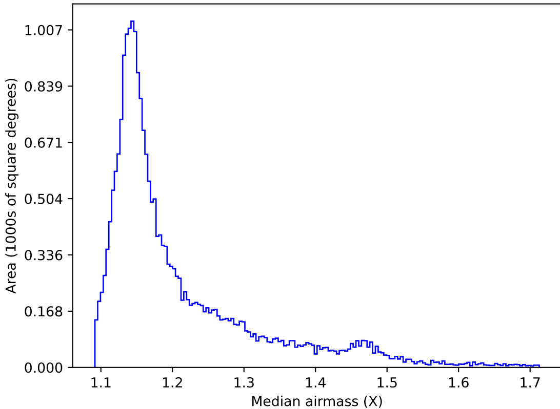
too_100_1v3.4_10yrs All sky y band: Median airmass
