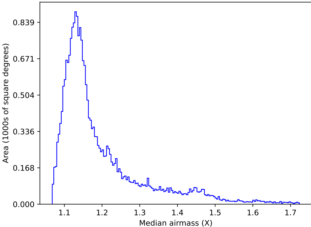
too_100_1v3.4_10yrs All sky u band: Median airmass
