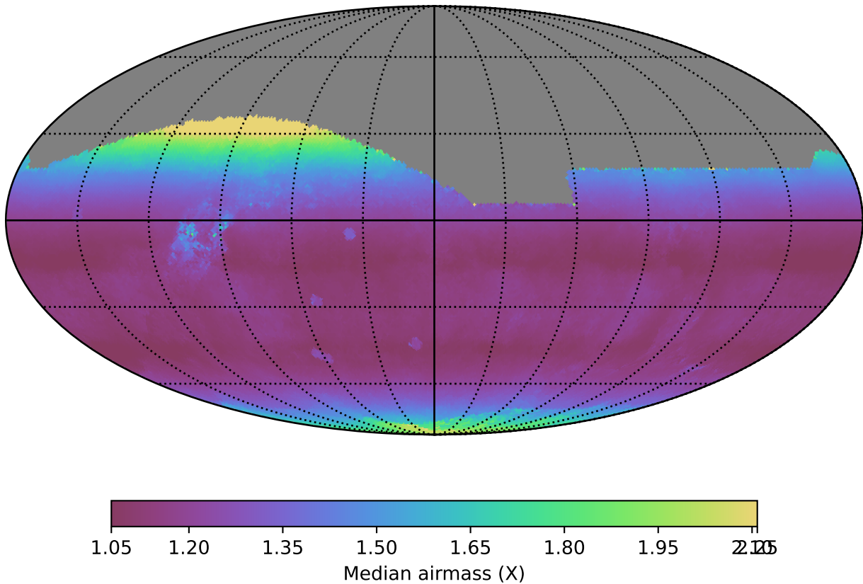
too_100_1v3.4_10yrs All sky r band: Median airmass
