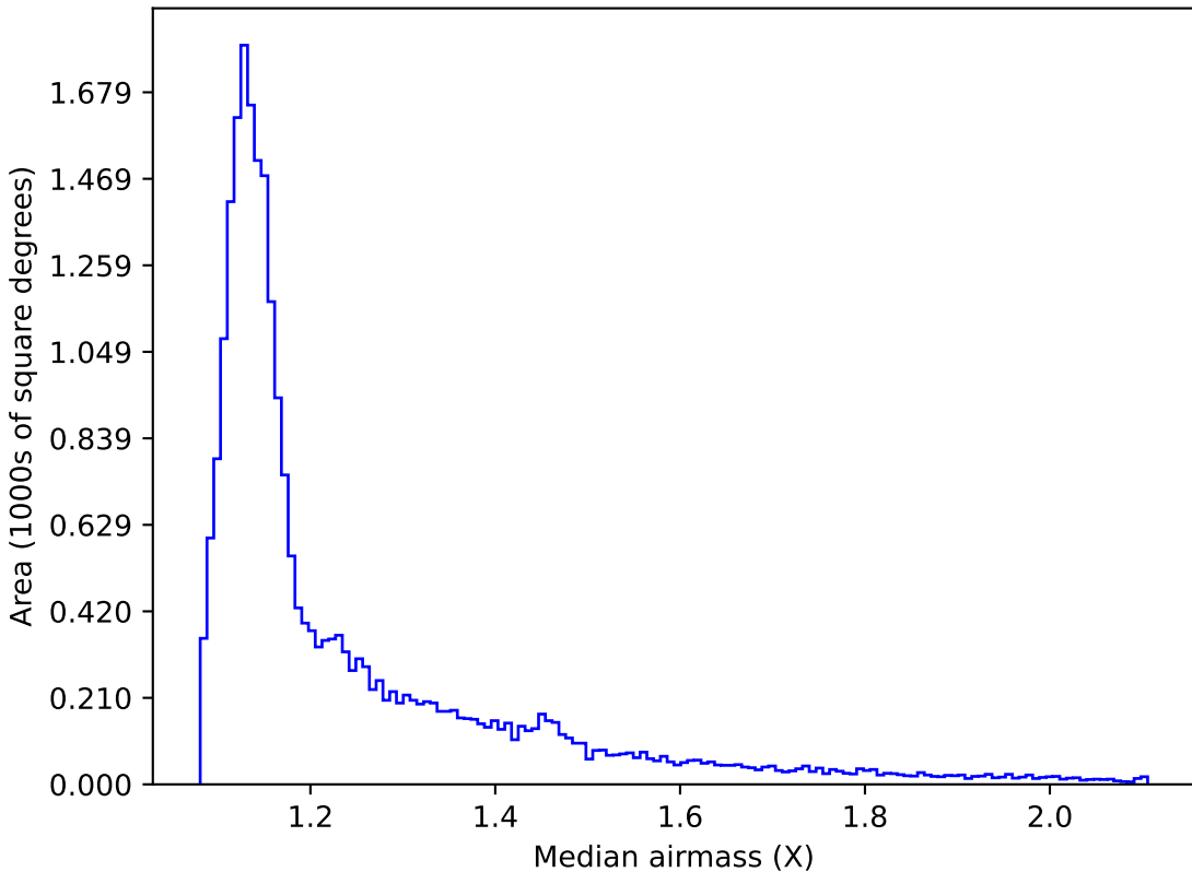
too_100_1v3.4_10yrs All sky i band: Median airmass
