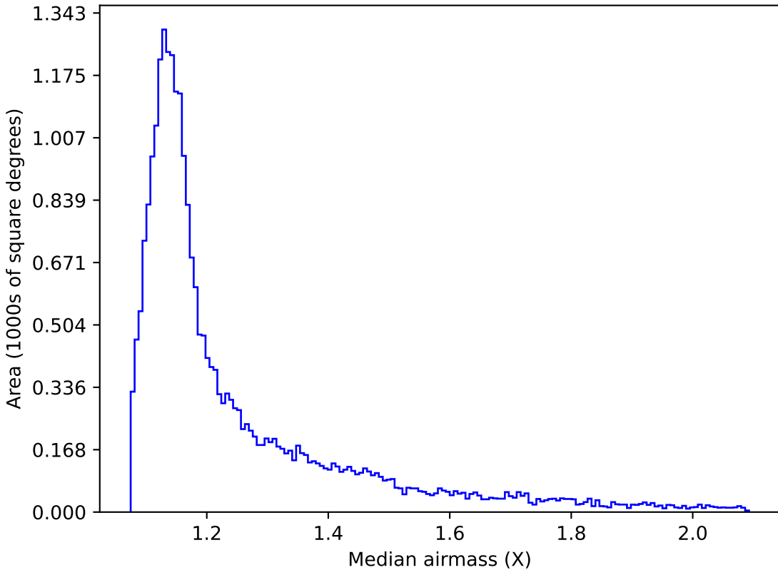
too_100_1v3.4_10yrs All sky g band: Median airmass
