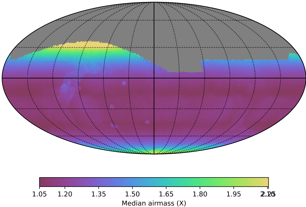
too_100_1v3.4_10yrs All sky all bands: Median airmass
