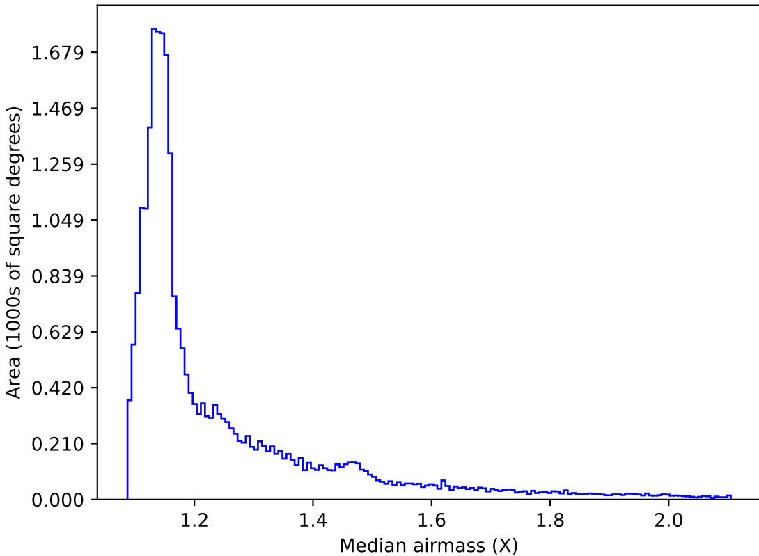
too_100_1v3.4_10yrs All sky all bands: Median airmass
