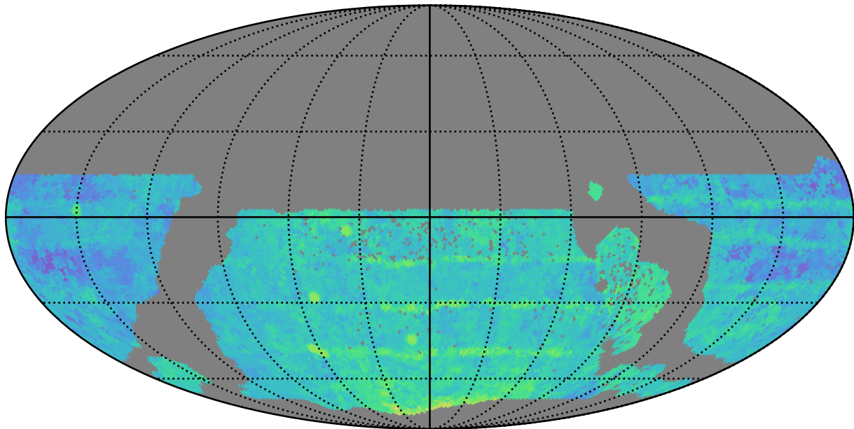
too_100_1v3.4_10yrs WFD z band: Median Season Length
